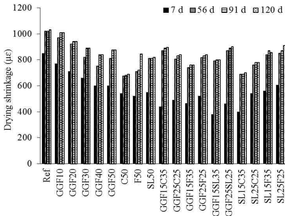
Figure 4.11 Drying shrinkage results ( \mu\epsilon )
