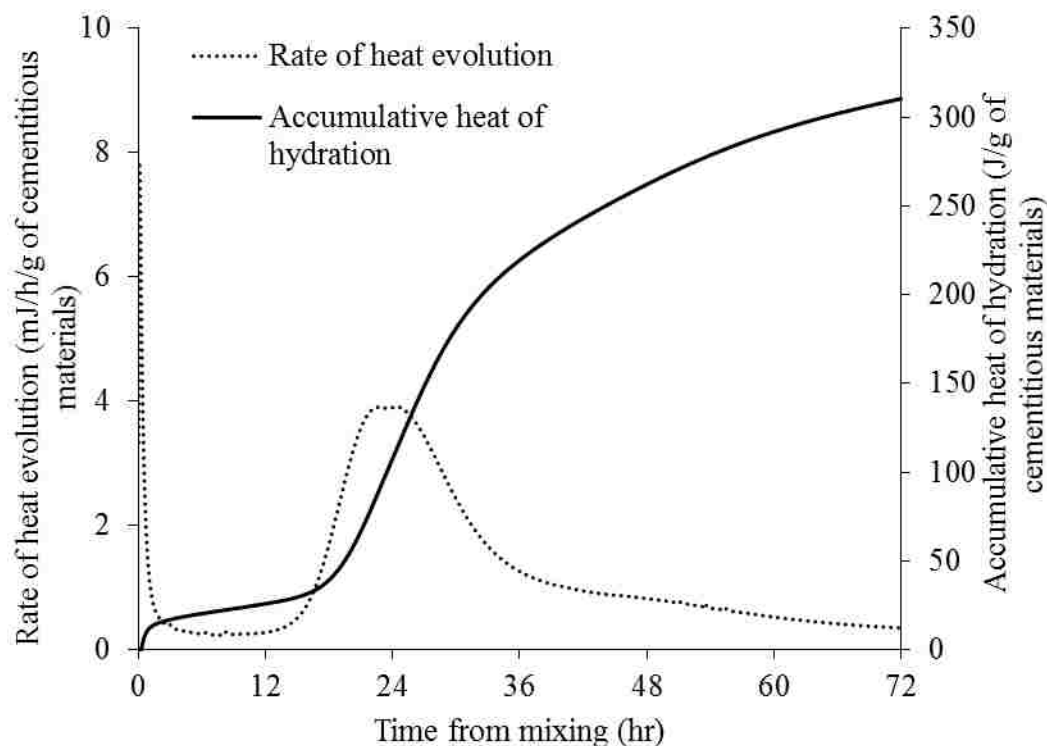
Figure 4.6 Calorimetry measurement of the Reference mixture (100% OPC)
