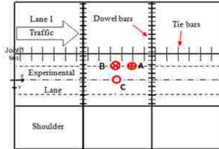
Figure 10.5 Schematic view of the pavement panels
