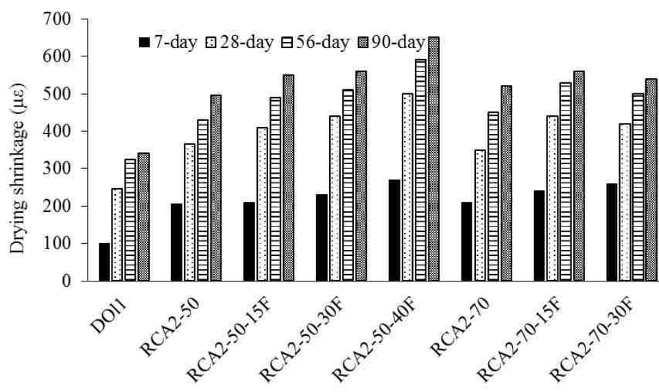
Figure 7.11 Effect of fine RCA on shrinkage of concrete made with 50% and 70% coarse RCA2
