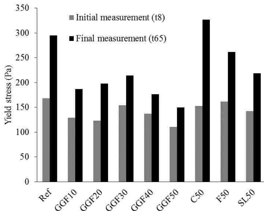
Figure 4.3 Variations in yield stress of the Reference and binary mixtures
