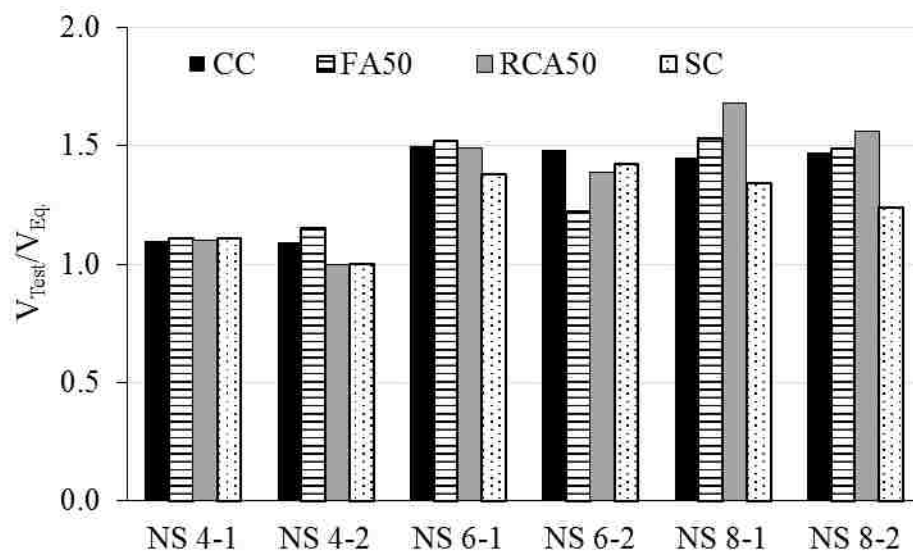
Figure 5 Comparing experiment-to-code values derived from ACI-318 (2011)
