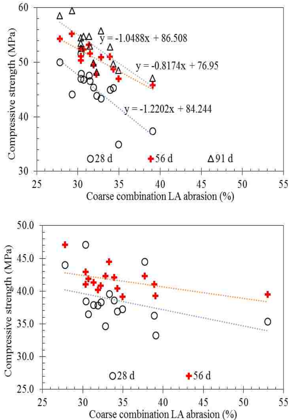
Figure 5.5 Effect of combined coarse aggregate LA abrasion on compressive strength; Top: ternary mixtures, Bot.: binary mixtures
